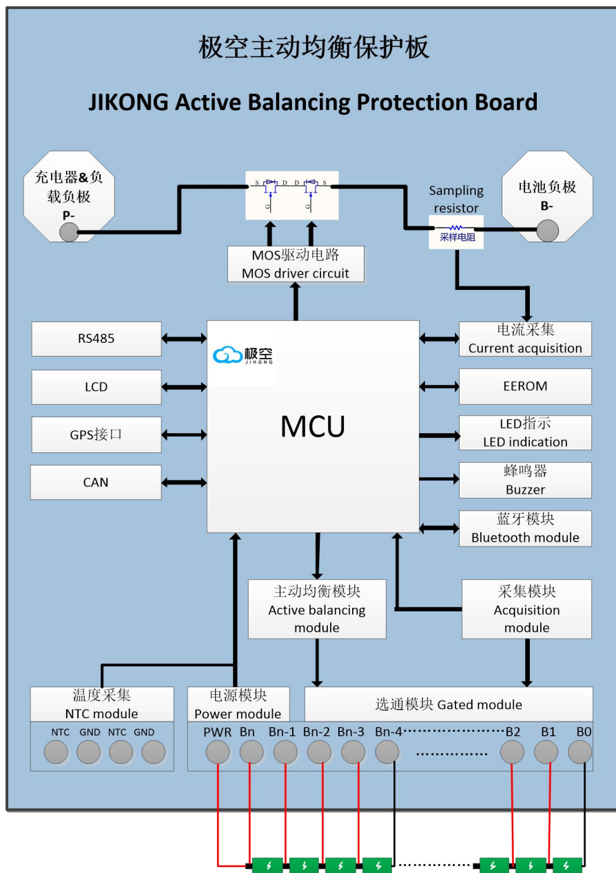
JK-BD4A17S/20S-4P 结构框图
