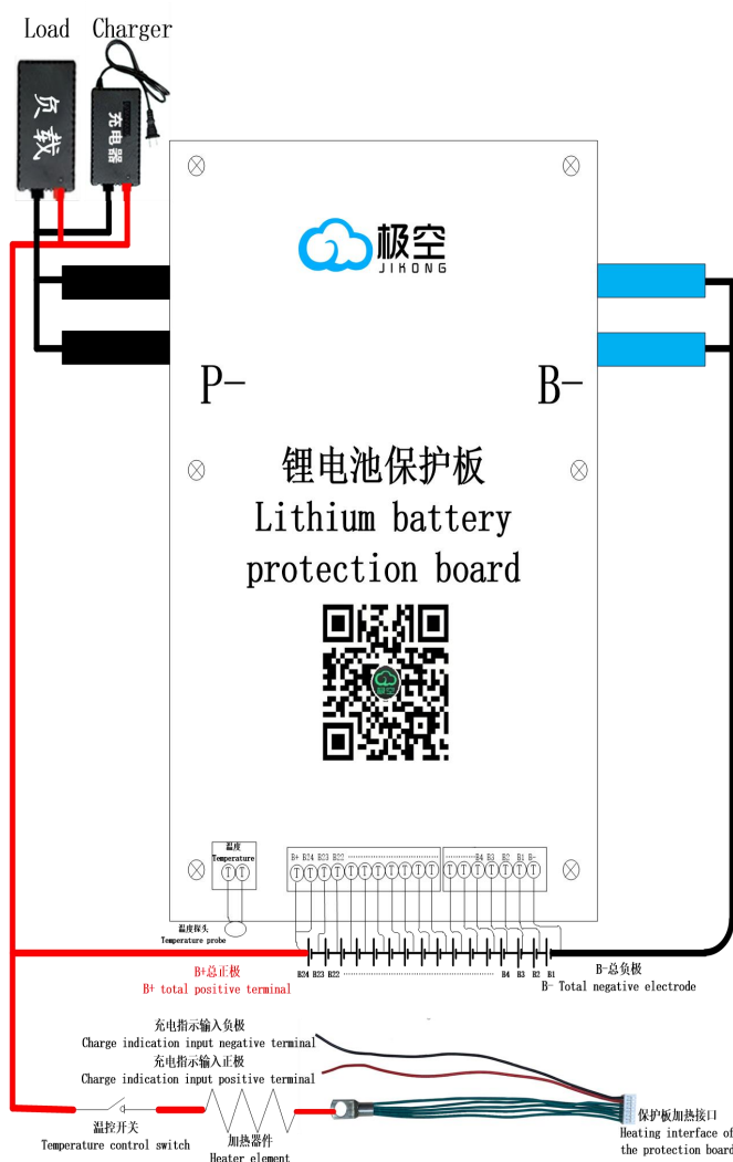
JK-BD6A20/24S-12P-24S接线图
