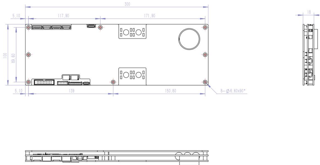
JK-PB1/2A16S-10/15/20P 外形尺寸 Dimensions of JK-PB1/2A16S-10/15/20P
