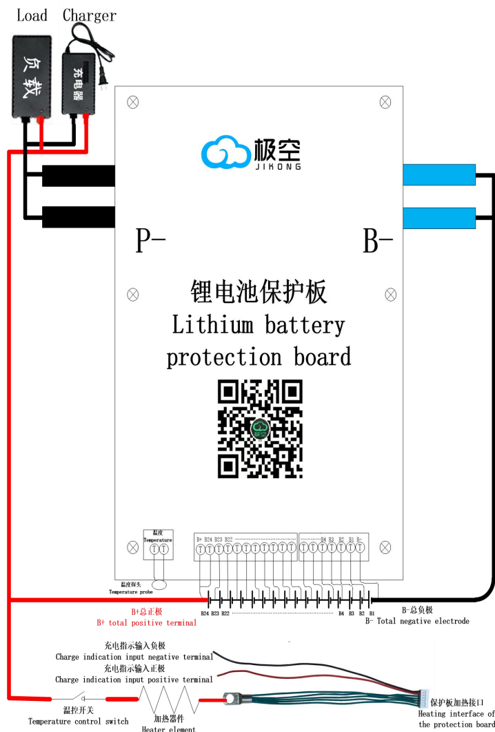
JK-BD6AxxS-15P/20P-24S接线图
